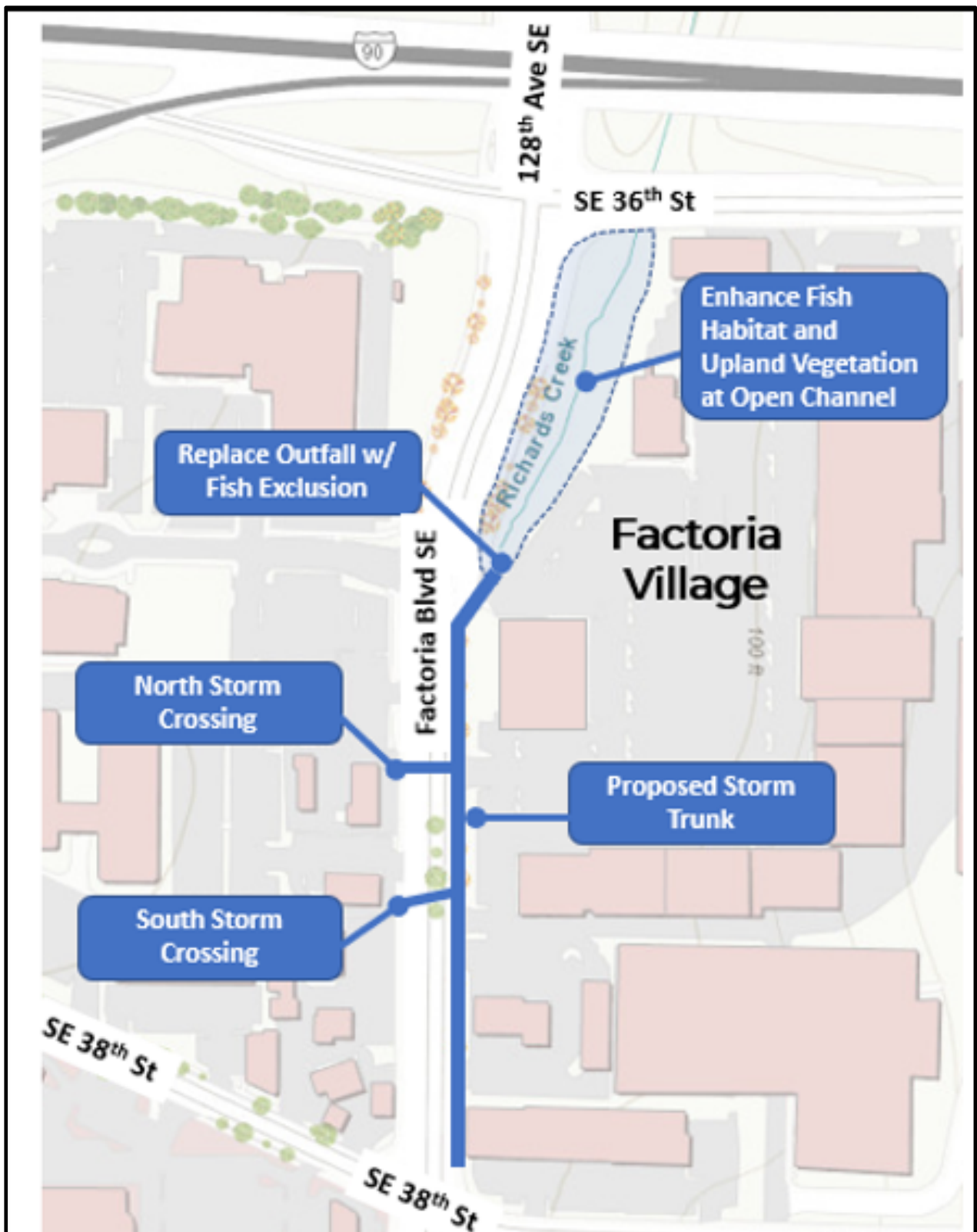
Figure 2. Factoria Boulevard Storm Conveyance Improvements Project Site Map and Proposed Improvements
