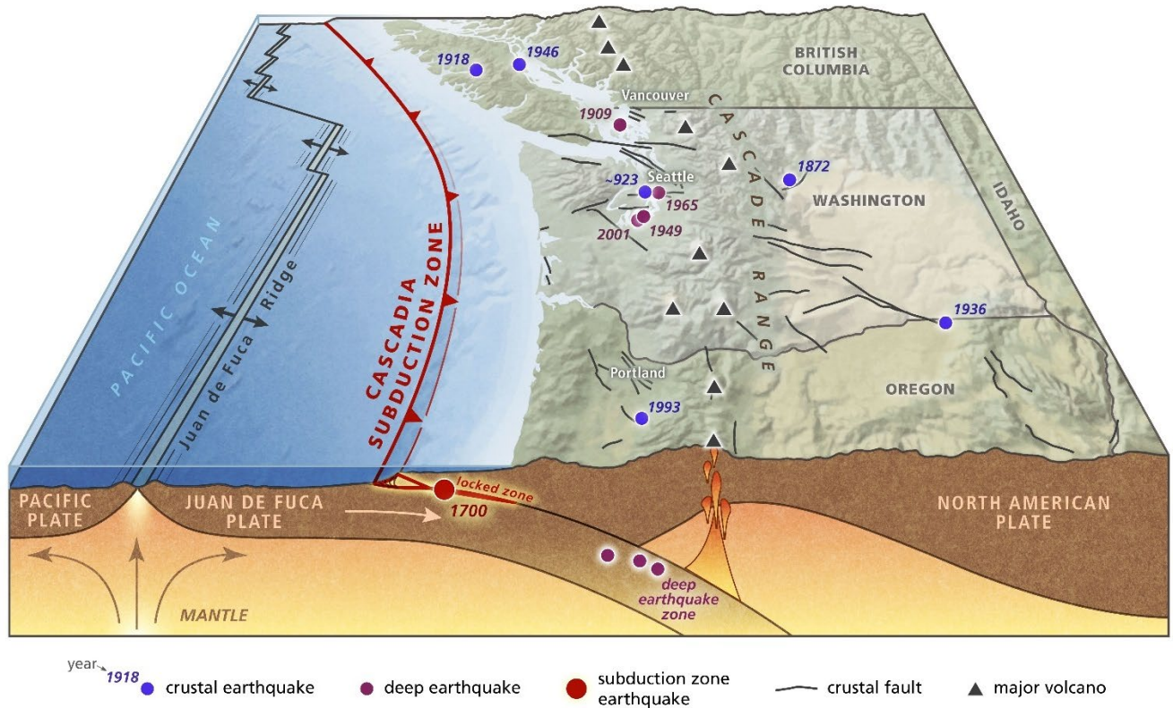
Figure 9-1 Earthquake sources and past events
