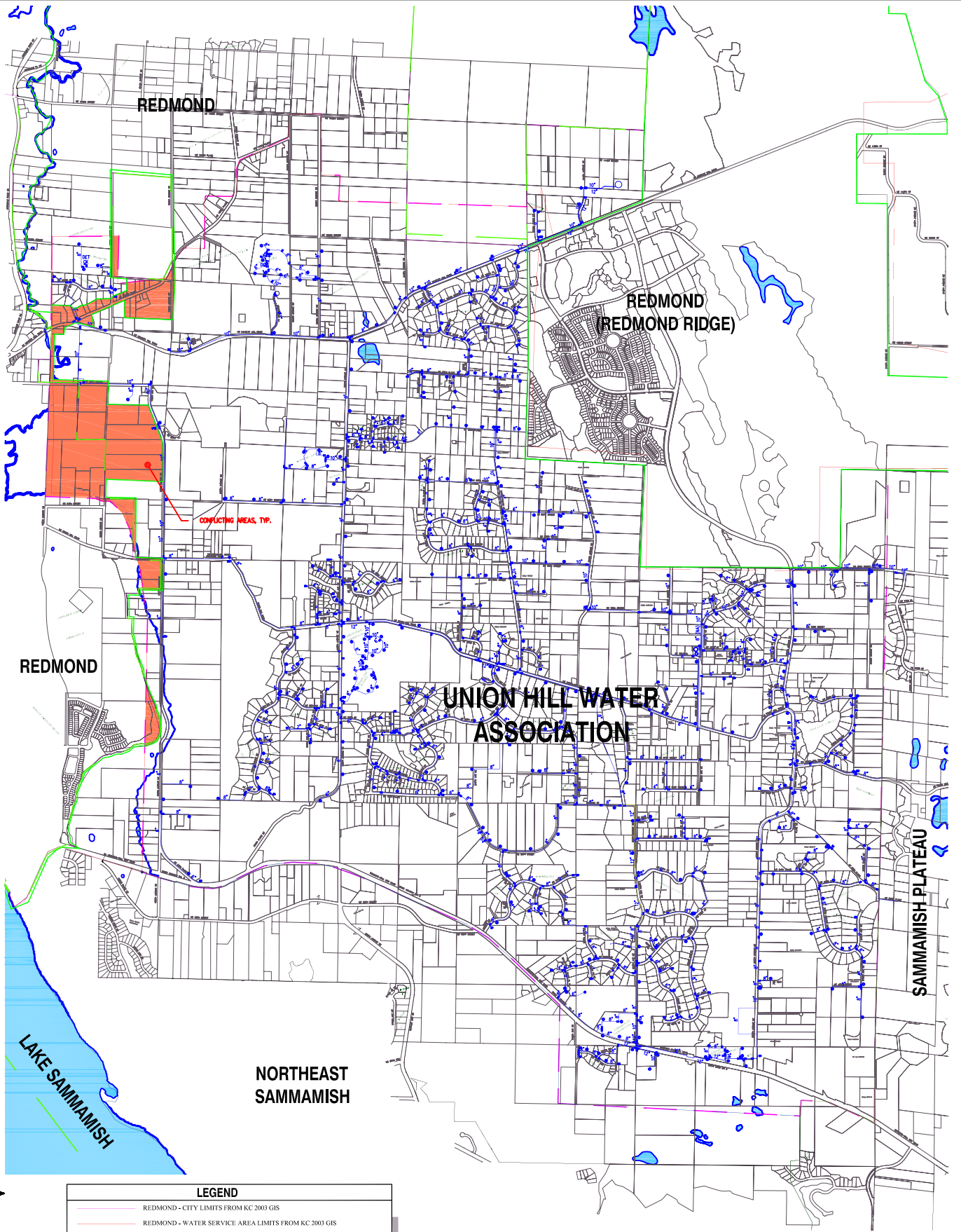
FIGURE 1-2: SERVICE AREA AND ADJACENT SYSTEMS
