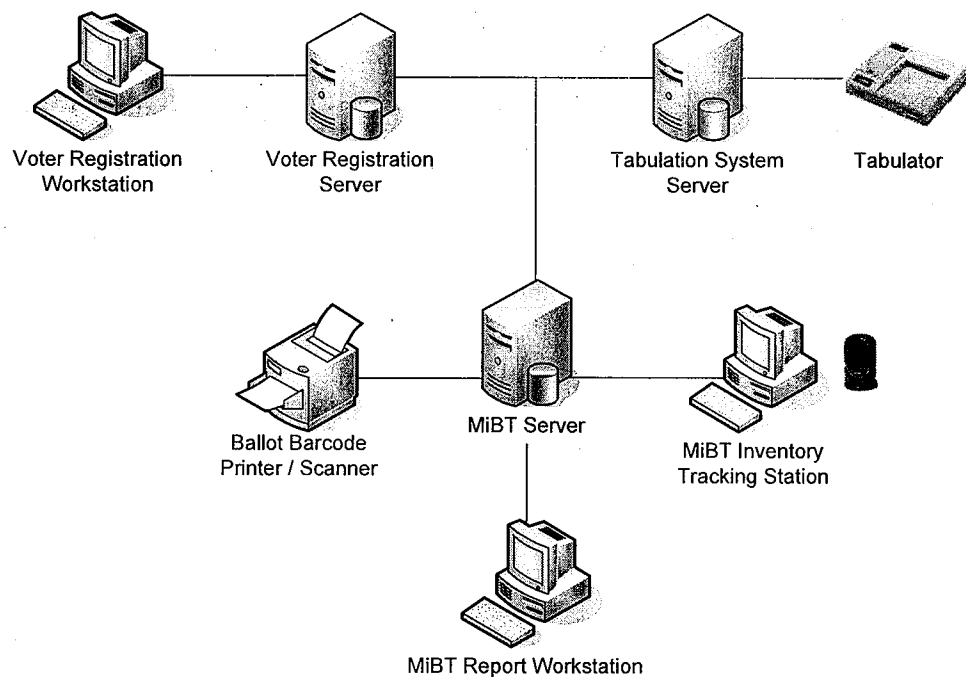
System Diagram
