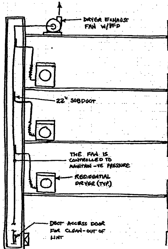
Dryer Exhaust Riser
