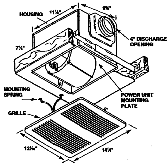
Bathroom Forced Air Return Terminal (FART) Fan
