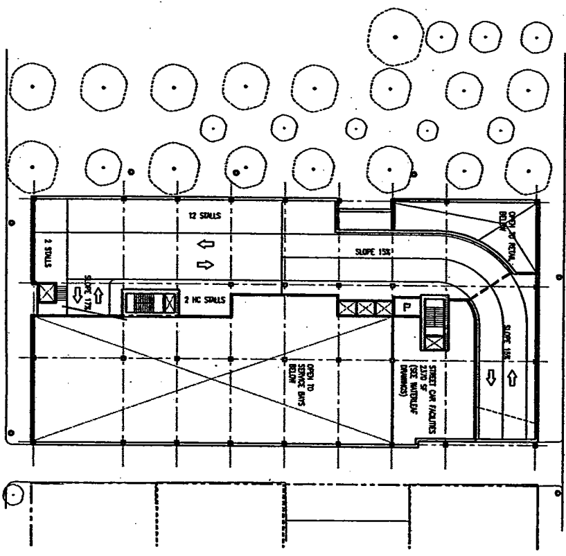
1 LEVEL 2 FLOOR PLAN - OPTION A
