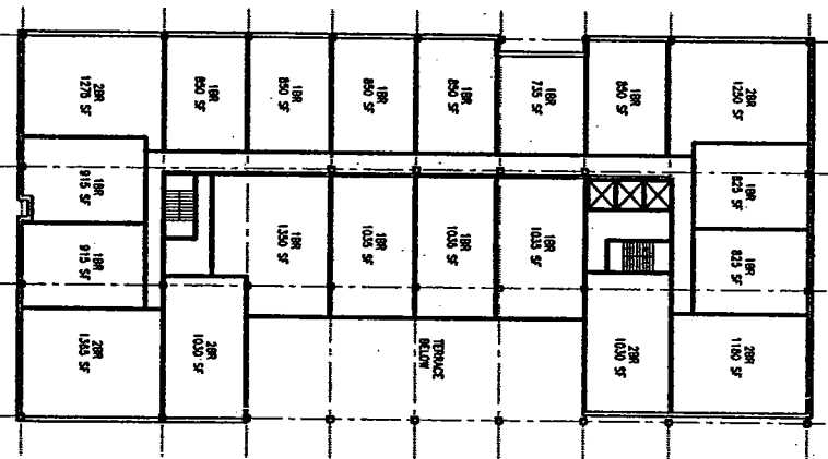
2 TYP. HOUSING FLOOR PLAN - CORRIDOR OPTION APPROX. 24,735 GSF, 20 UNITS 1" = 3/8"
