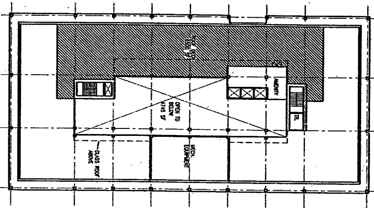
2 ROOF PLAN - NATURAL VENTILATION OPTION
