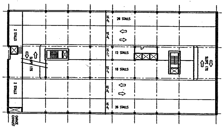
2 TYP. PARKING FLOOR PLAN - OPTION A
