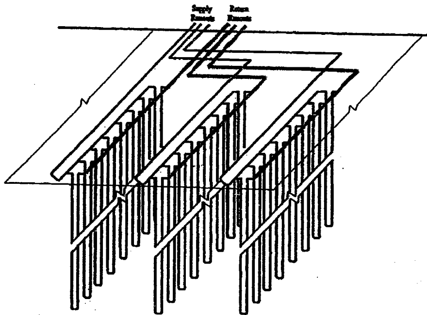
Sample Vertical Heat Exchanger
