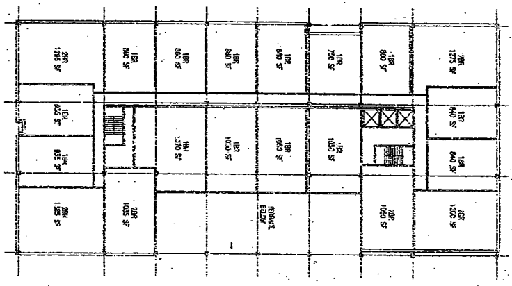
2 TYP. HOUSING FLOOR PLAN - TERRACE OPTION 1/2000 CSF, 19 UNITS
