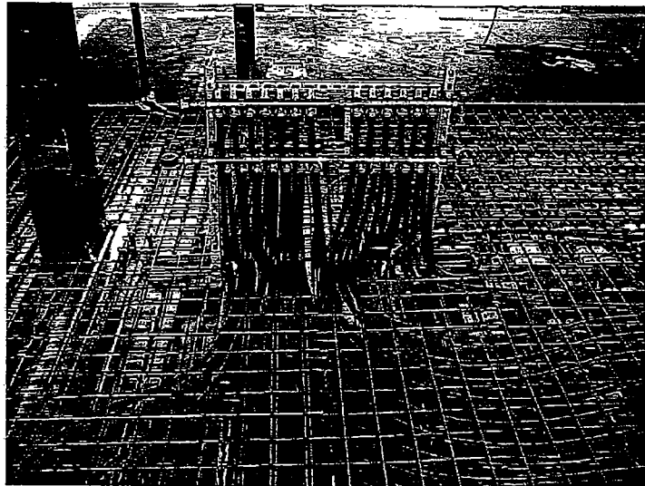
Radiant Floor Header and PEX Tubing
