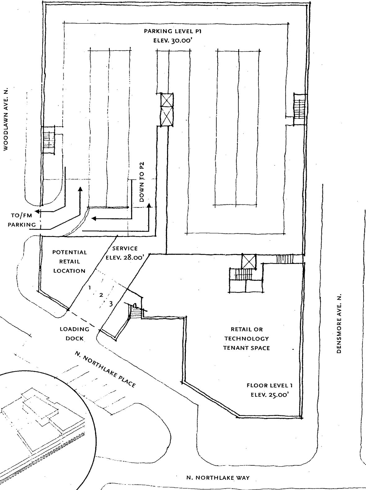
PLAN @ 1ST FLOOR - NORTHLAKE WAY ACCESS
