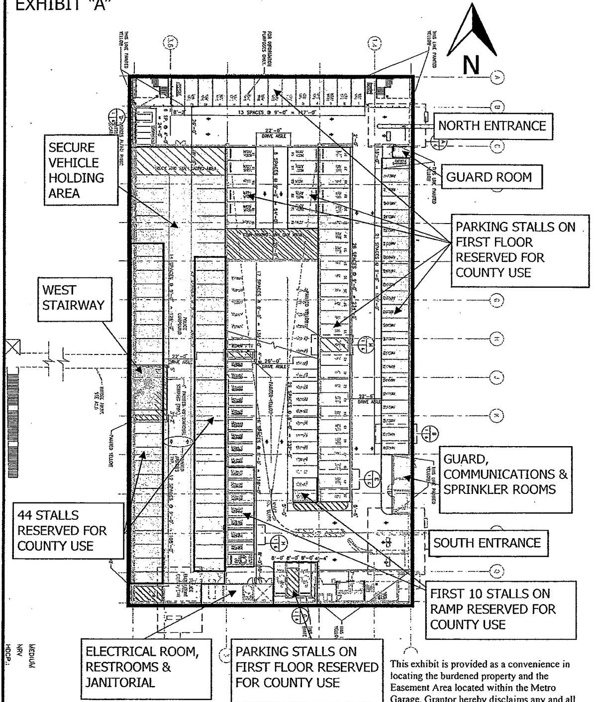
METRO GARAGE—LEVEL 1 LAYOUT
